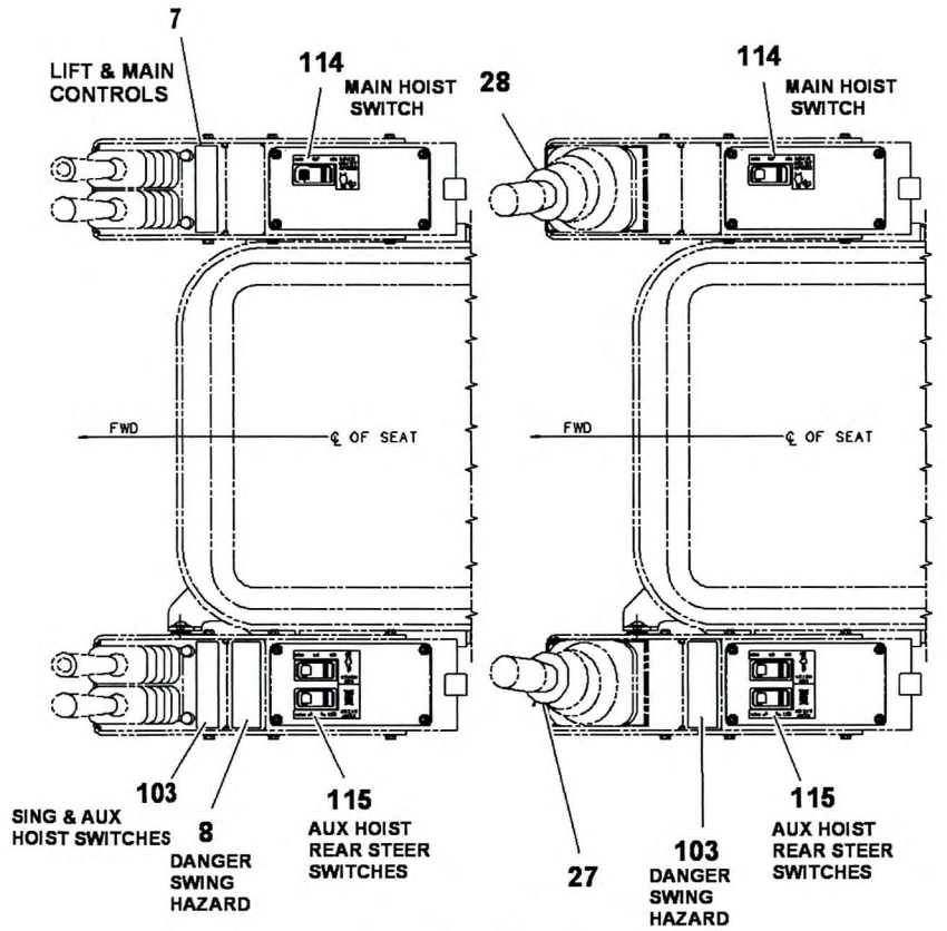
DUAL AXIS CONTROLLERS (CE)
