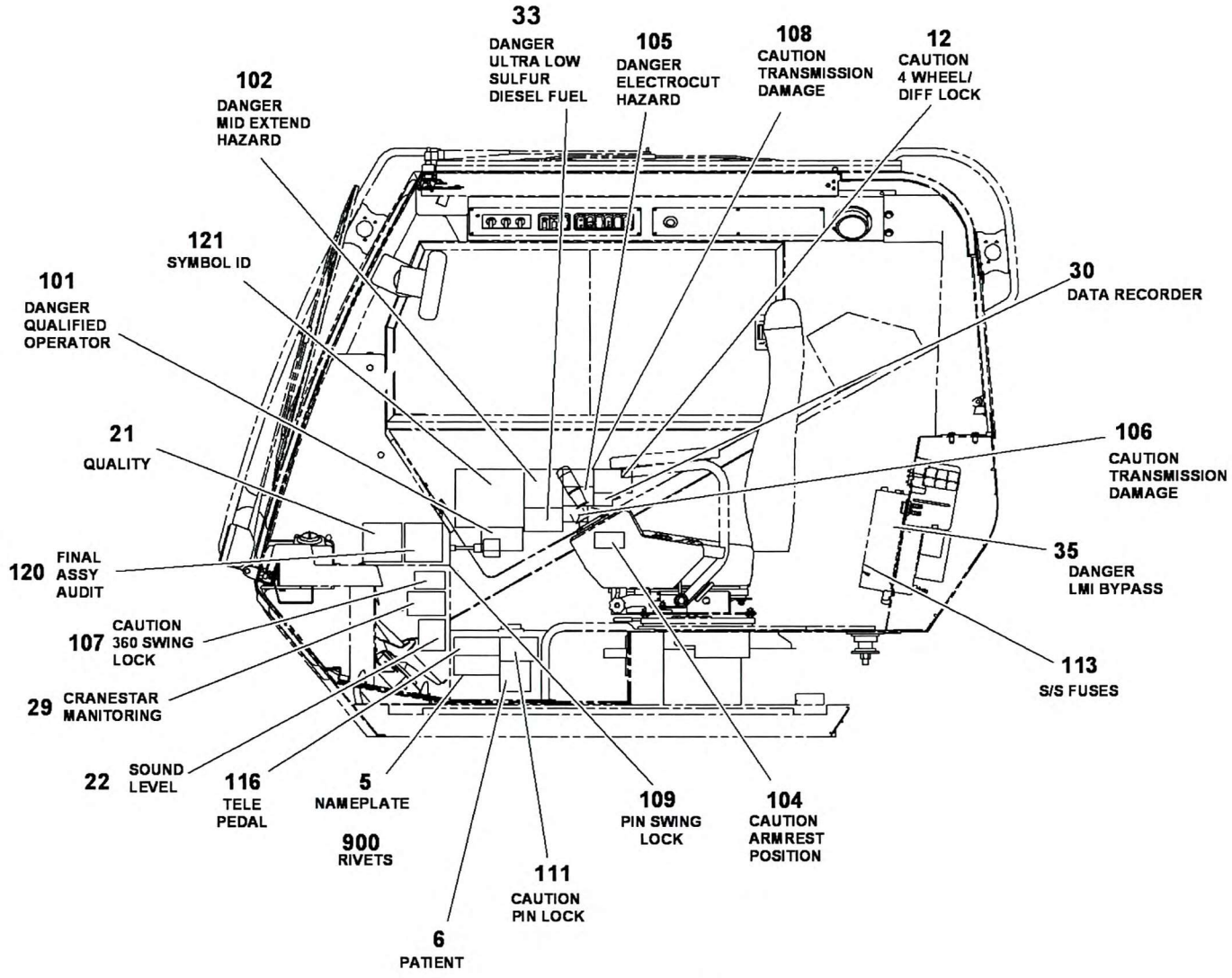
CAB INSIDE VIEW
