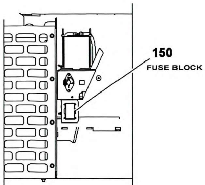
BATTERY COMPARTMENT
